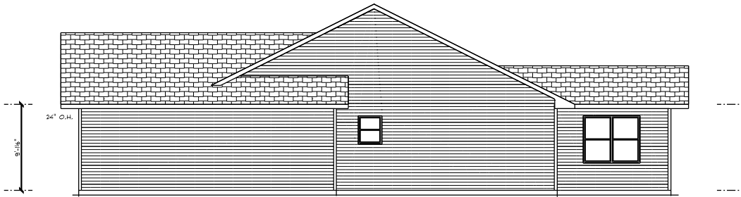
RIGHT ELEVATION 1/8" = 1'-0"
